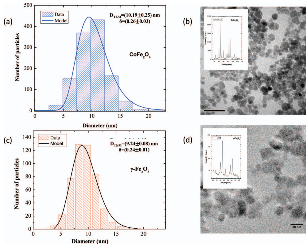
FIG. 2. Morphological characterization. TEM micrographs for cobalt ferrite (b) and maghemite (d); the inset illustrates data from X Ray diffraction. The corresponding size distribution histograms are shown in images (a) and (c) respectively, together with a lognormal distribution fit.
