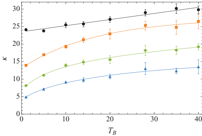
FIG. 6. (Color online) Heat conductivity \kappa = JL/\Delta T as a function of the temperature T = T_B of the colder reservoir for several values of \lambda . From top to bottom \lambda = 0, 0.02, 0.05, and 0.1 . All results were obtained for a chain of size L = 500 and by using the same value of the difference in temperature of the reservoirs, \Delta T = 1 . The solid lines are a guide to the eye.
