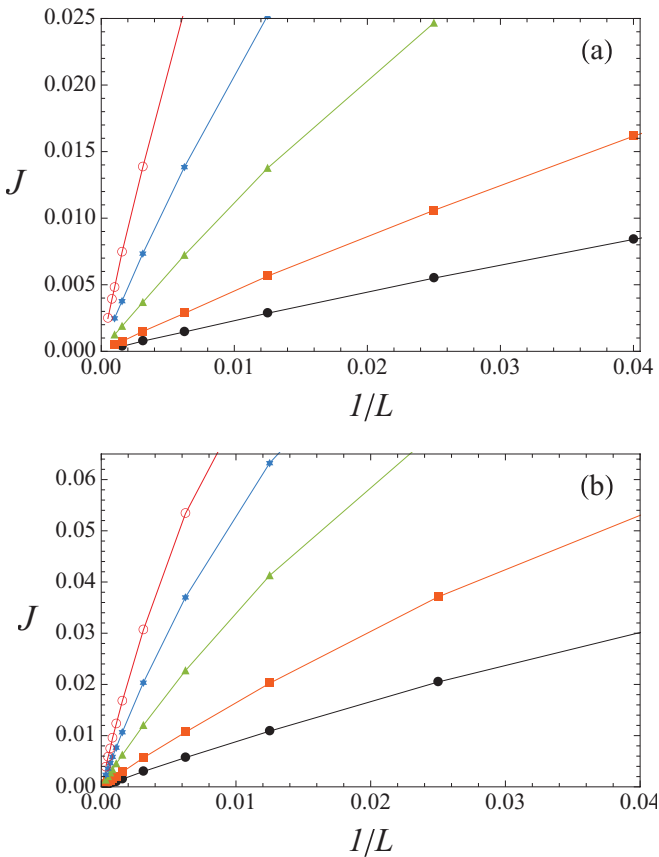
FIG. 2. (Color online) Heat flux J as a function of the inverse of the system size L for several values of \lambda for (a) the harmonic chain and (b) the anharmonic chain. In both cases, from top to bottom, \lambda = 0.05, 0.1, 0.2, 0.5 , and 1 . The temperatures of the reservoirs are T_A = 2 and T_B = 1 . In (a) the solid lines are exact results.
