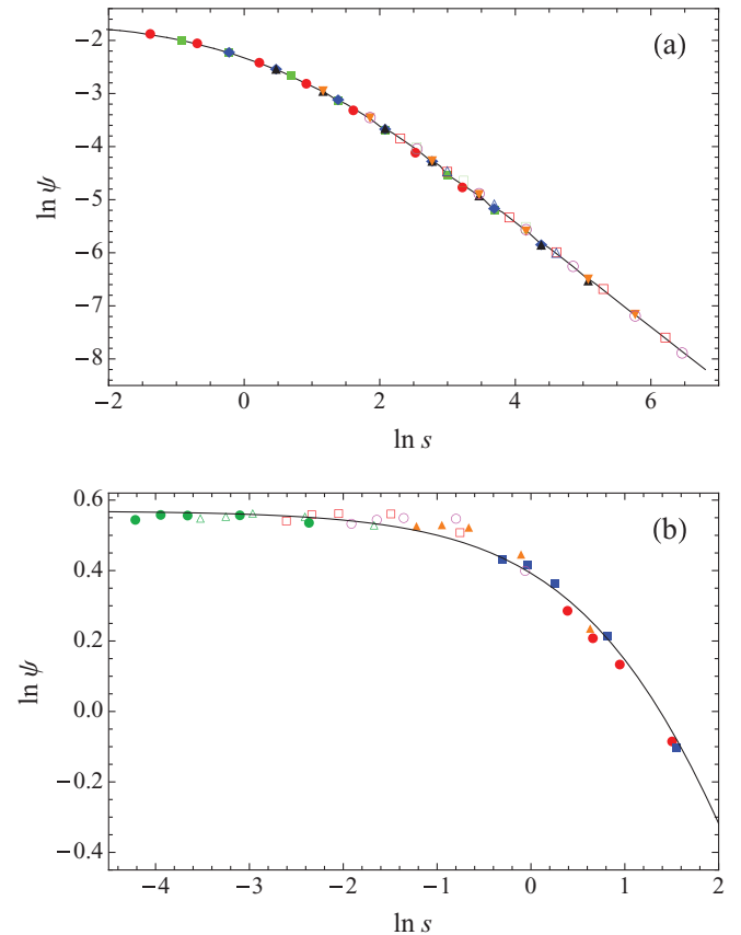
FIG. 5. (Color online) Data collapse obtained from the numerical results of the heat conductivity \kappa obtained from several values of \lambda and L corresponding to (a) the harmonic case and (b) the anharmonic case, where \Psi = \kappa/L^a and s = \lambda L^{a/b} . The solid line in (a) is described by expression (17) with A = 1/4 and B = 3/2 . In (b), the solid line is a guide to the eye. The temperatures of the reservoirs are T_A = 2 and T_B = 1 . Points with the same symbol correspond to the same value of \lambda .
