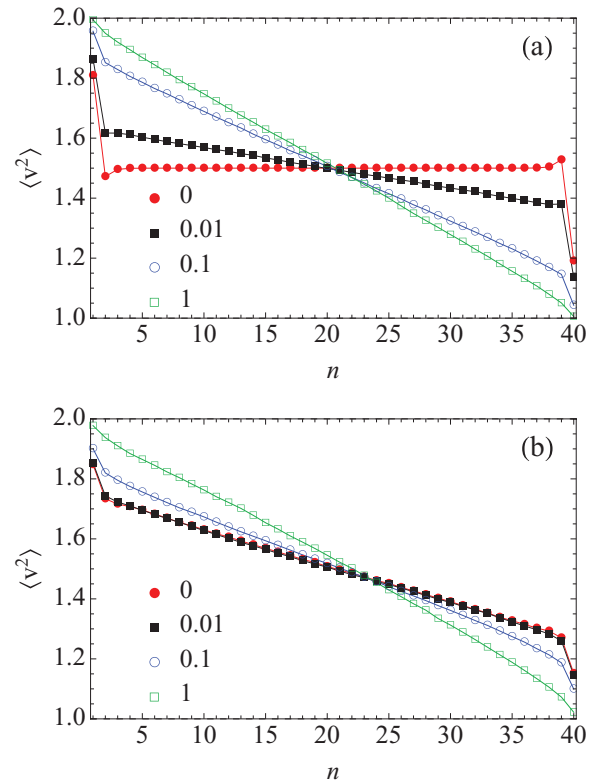
FIG. 1. (Color online) Average square velocity \langle v_n^2 \rangle of the particles as a function of the position n on the chain, which is in contact with heat reservoirs at temperatures T_A = 2 and T_B = 1 . Results are given for a chain of L = 40 particles for the values of \lambda indicated for the (a) harmonic case and (b) anharmonic case. In (a) the solid lines are exact results.
