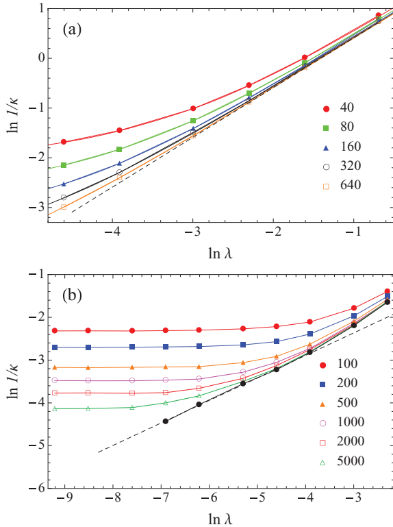
FIG. 4. (Color online) Log-log plot of the reciprocal of the heat conductivity \kappa as a function of the collision noise \lambda for (a) the harmonic chain and (b) the anharmonic chain for several values of L . The temperatures of the reservoirs are T_A = 2 and T_B = 1 . In (a) the solid lines are exact results. The slope of the straight dashed line is b = 1 for (a) and b = 0.52 for (b). The lowest curve in both cases is an extrapolation obtained from finite values of L .
