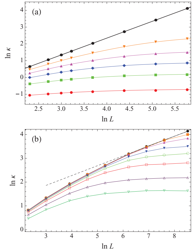
FIG. 3. (Color online) Log-log plot of the heat conductivity \kappa as a function of the system size L for (a) the harmonic chain and (b) the anharmonic chain. From top to bottom, \lambda = 0, 0.02, 0.05, 0.1, 0.2 , and 0.5 for (a) and \lambda = 0, 0.001, 0.002, 0.005, 0.01, 0.02, 0.05 , and 0.1 for (b). The temperatures of the reservoirs are T_A = 2 and T_B = 1 . In (a), the solid lines are exact results, and the slope of the straight line corresponding to \lambda = 0 is a = 1 . In (b), the slope of the straight line (shown as a dashed line) fitted to the data points with large L corresponding to \lambda = 0 gives a = 0.42 .
