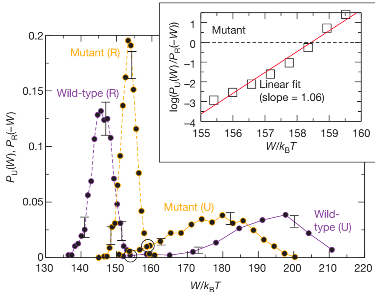
Figure 3 | Free-energy recovery and test of the CFT for non-gaussian work distributions. Experiments were carried out on the wild-type and mutant S15 three-helix junction without \text{Mg}^{2+} . Unfolding (continuous lines) and refolding (dashed lines) work distributions. Statistics: 900 pulls and two molecules (wild type, purple); 1,200 pulls and five molecules (mutant type, orange). Crossings between distributions are indicated by black circles. Work histograms were found to be reproducible among different molecules (error bars indicating the range of variability). Inset, test of the CFT for the mutant. Data have been linearly interpolated between contiguous bins of the unfolding and refolding work distributions.
